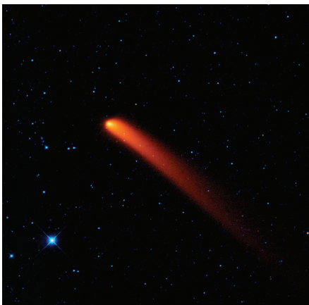
Comet Siding Spring
