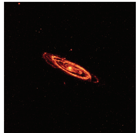
Andromeda Galaxy
