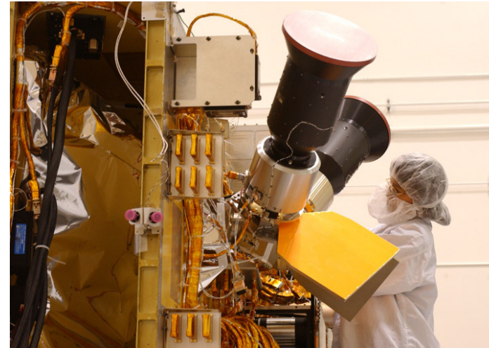
4 Star Trackers
