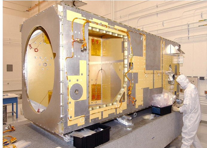
1 Bus Structure
