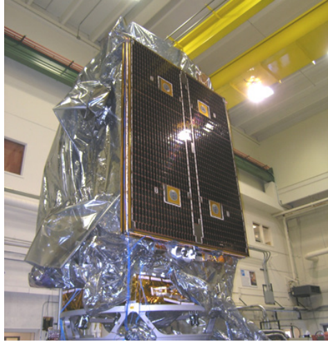
13 Vibration Testing
