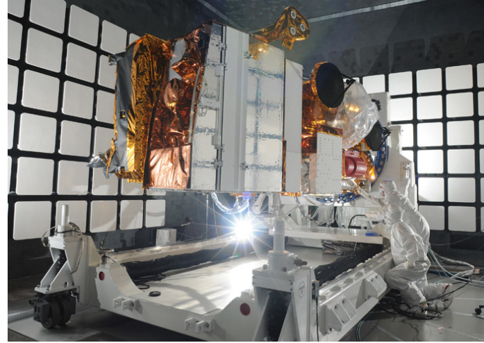
14 Electromagnetic Interference (EMI) Testing
