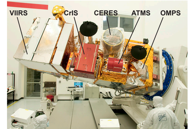
12 All Instruments Aboard
